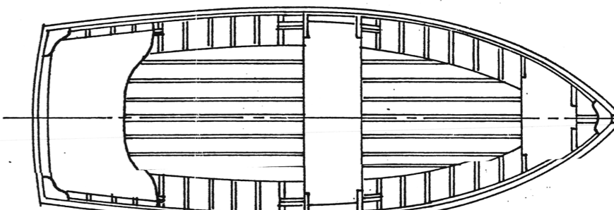
G.A. PLAN
