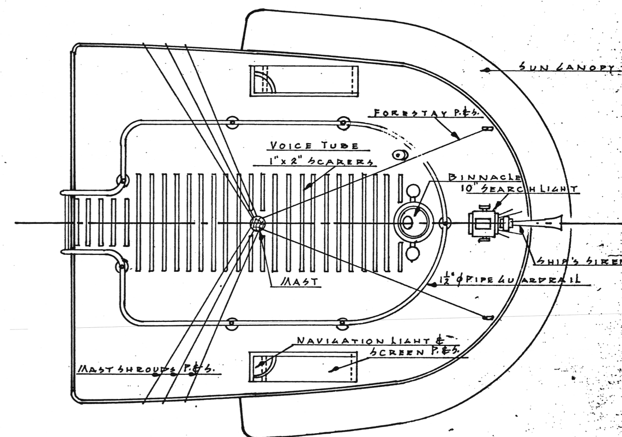
WHEEL HOUSE ROOF PLAN
