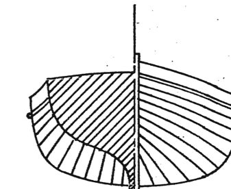
BODY PLAN
