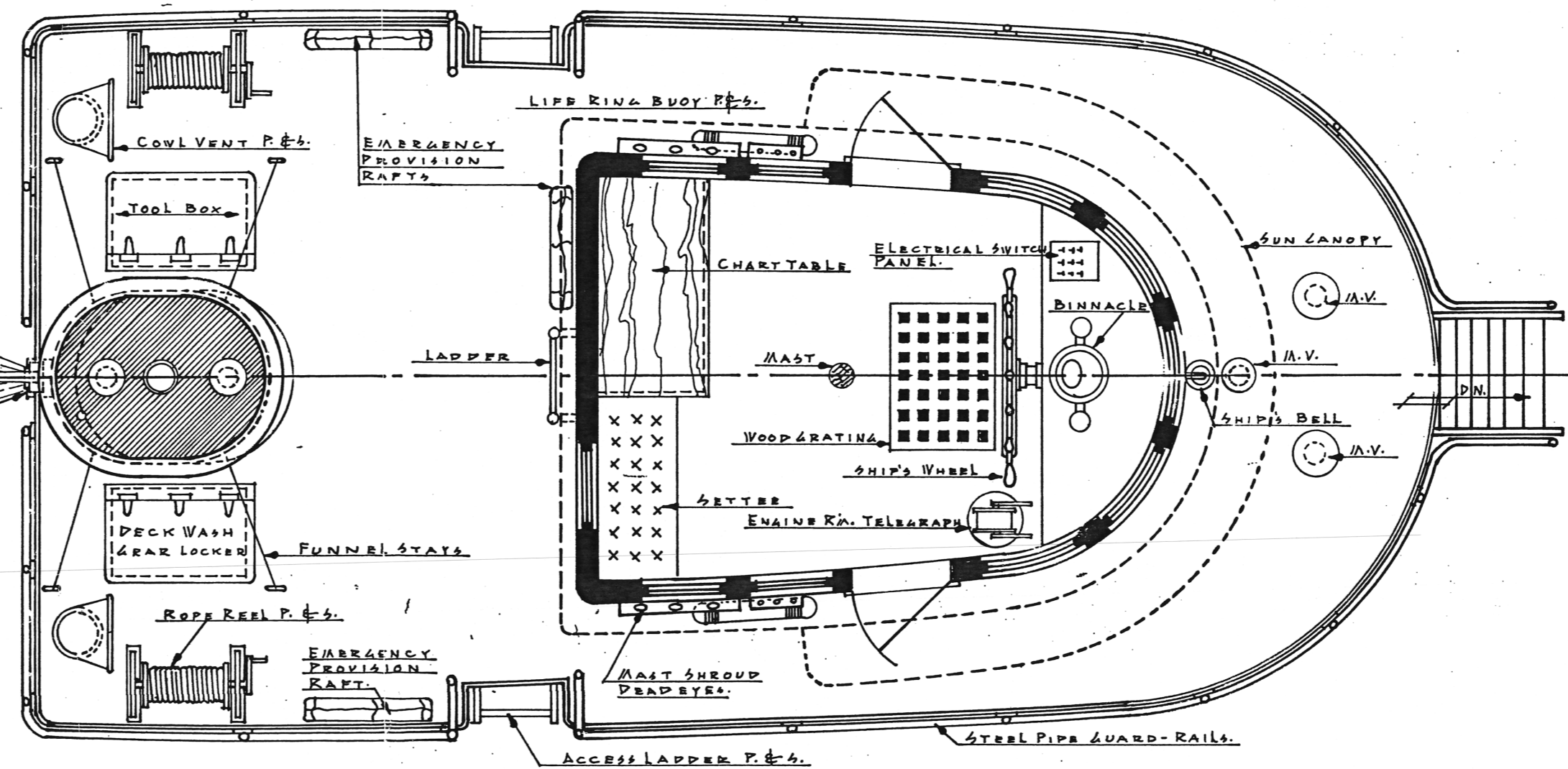
WHEEL HOUSE DECK PLAN
